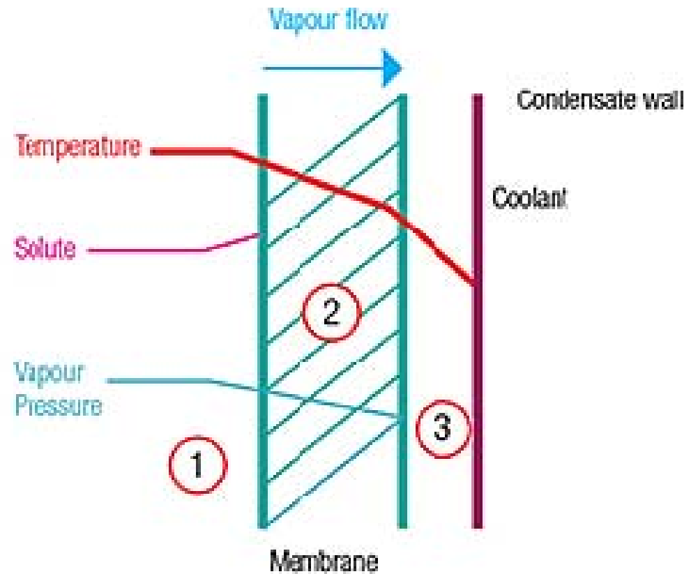
Profile diagram of air gap membrane distillation
